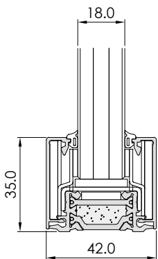
Vetrotech Contraflam 30
