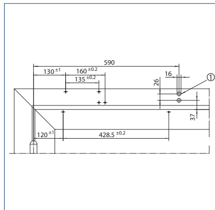
Fitting dimensions for left-hand door | 1 = line-feed 230 V
