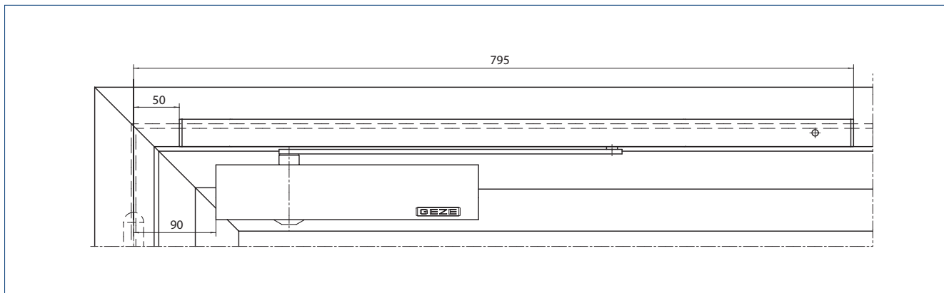
Installation example
