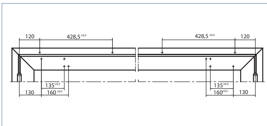
Fitting dimensions
