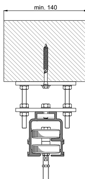
Montage an bauseitigem Holzbinder Installation on timber beam
